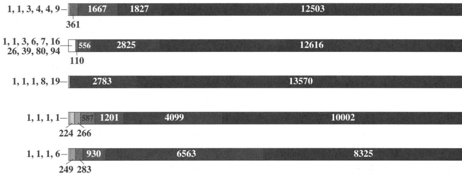
FIGURE 3. Factorization patterns for five pseudorandom polynomials of degree 16 383 in \mathbb{F}_2[x] .
